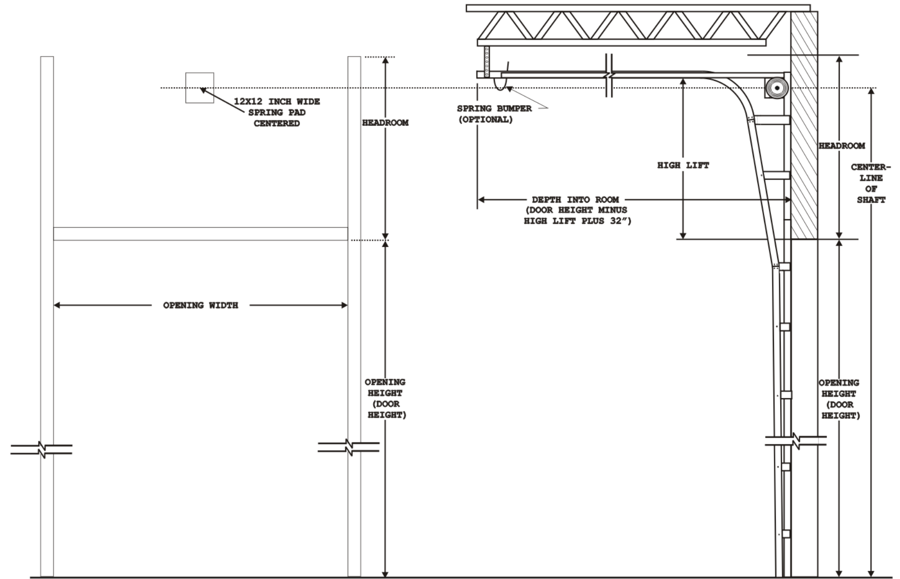
INTERIOR ELEVATION
