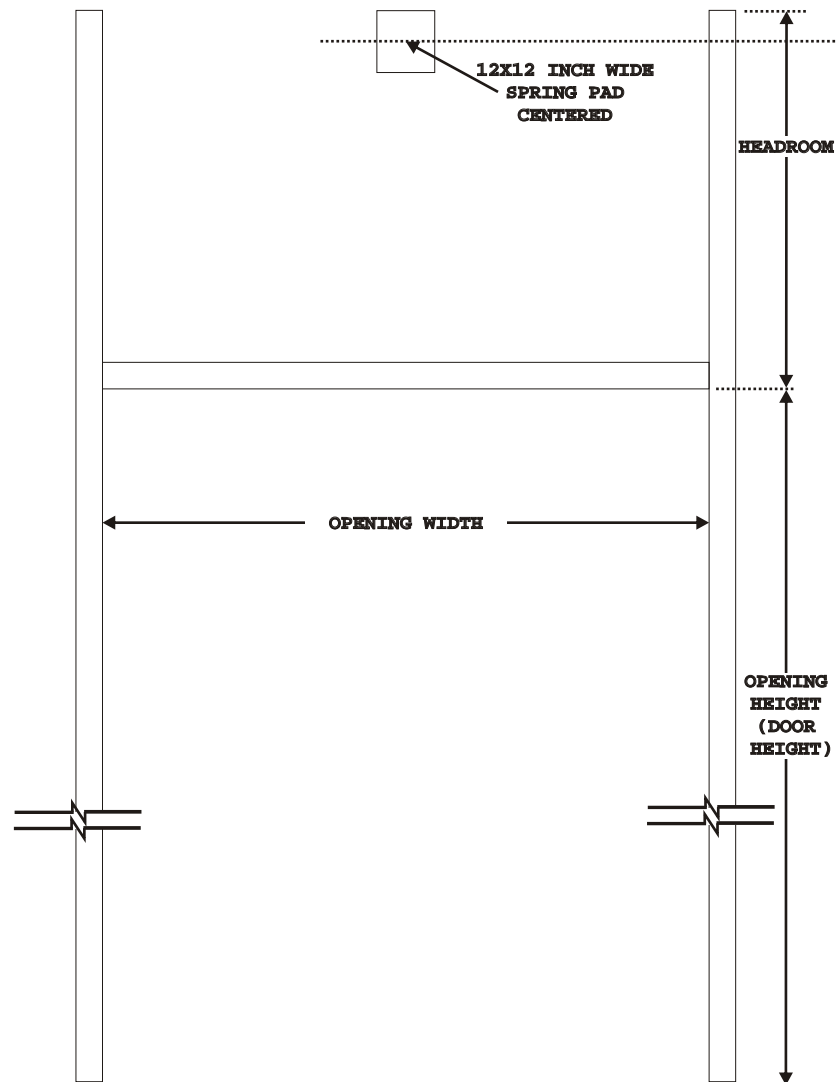
INTERIOR ELEVATION
