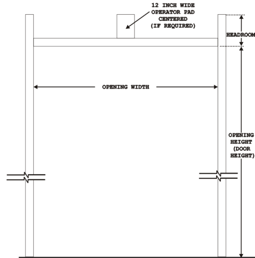
INTERIOR ELEVATION
