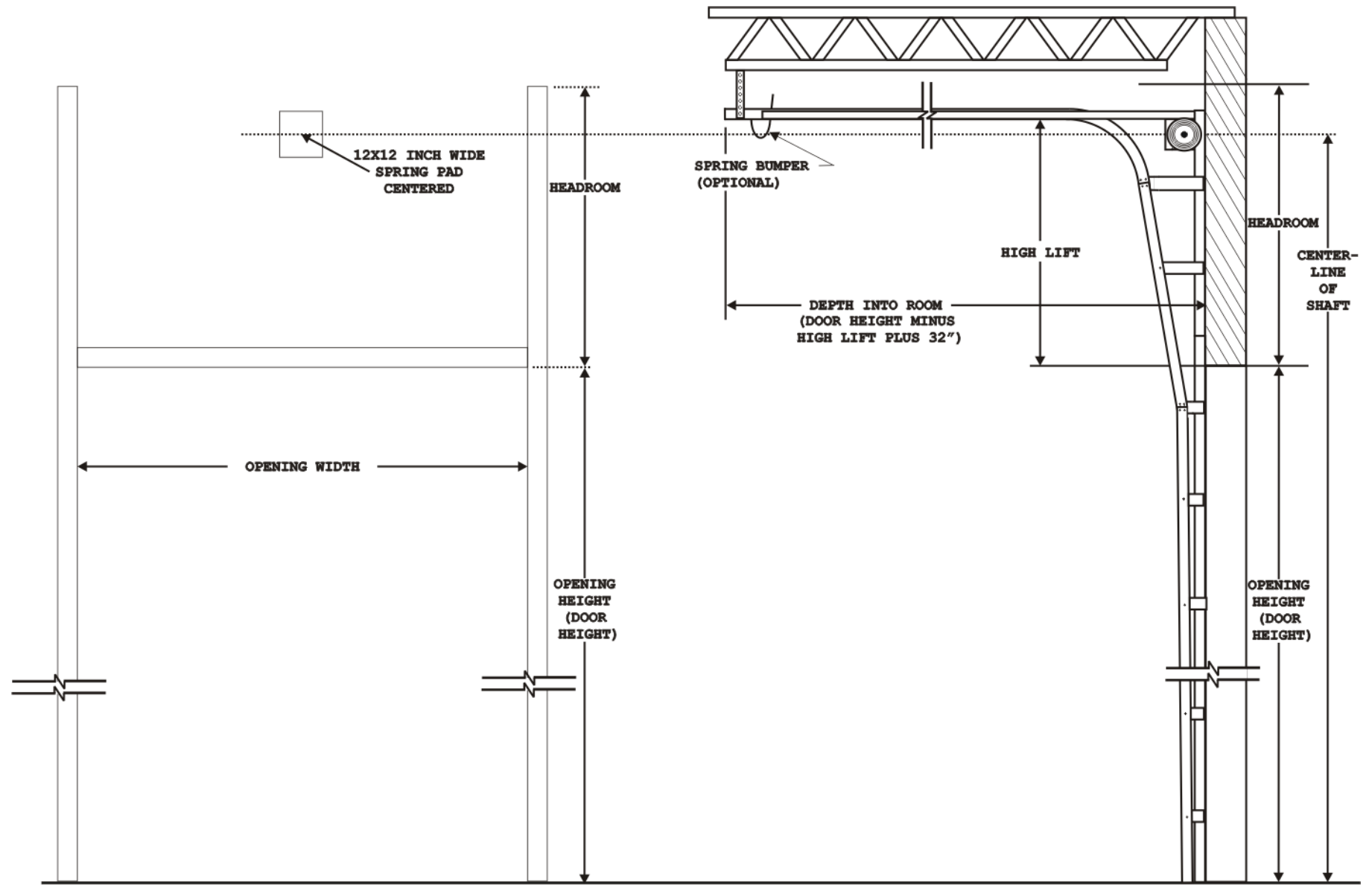
INTERIOR ELEVATION
