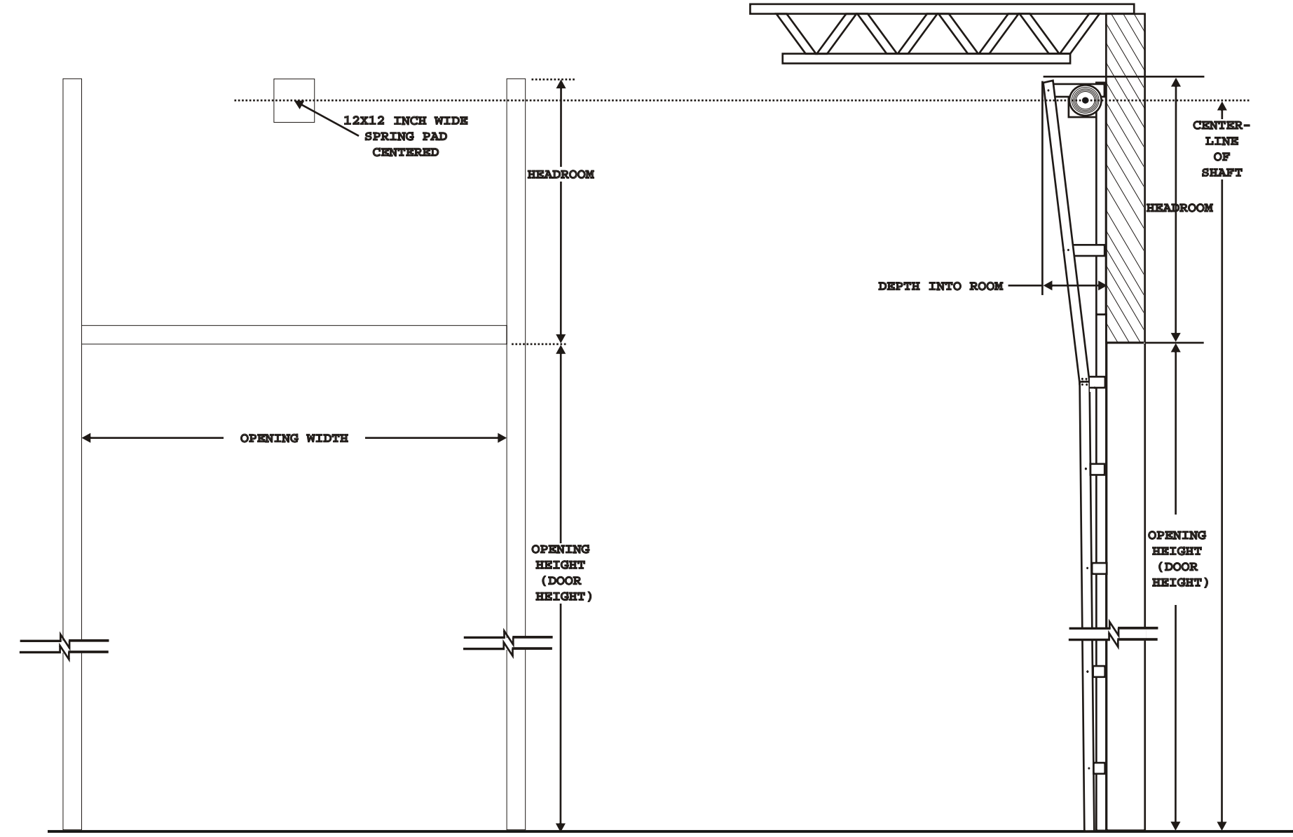
INTERIOR ELEVATION
