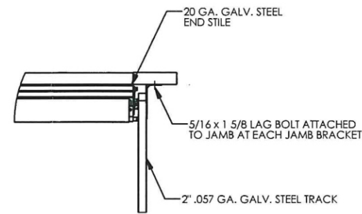
DETAIL E
