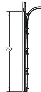
SECTION F-F SCALE 1 : 24
